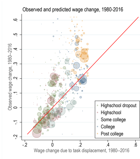
FIGURE 12: Predicted (horizontal axis) vs. observed (vertical axis) wage changes. The 45° line is shown in red. Marker sizes indicate the share of hours worked by each group and different colors indicate education levels. See text for variable definitions.
