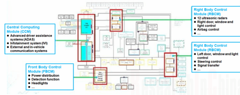
Zone Controller Configuration of Tesla Model 3
