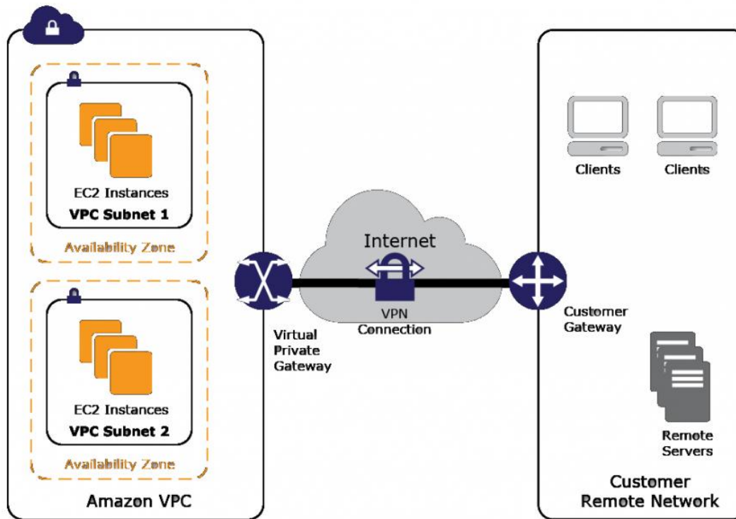
Figure 1: AWS managed VPN
