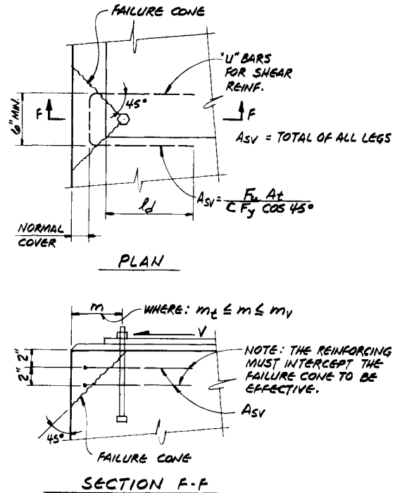
Fig. 3. Shear reinforcement
