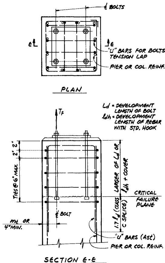
Fig. 4. Tension lap
