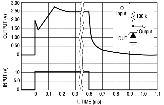
Figure 12. Response Time
