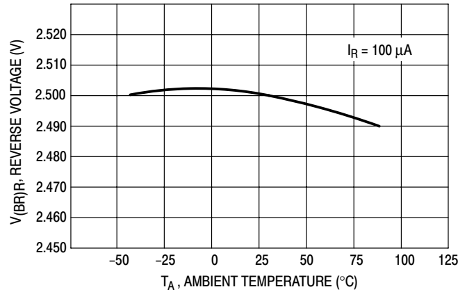
Figure 10. Temperature Drift
