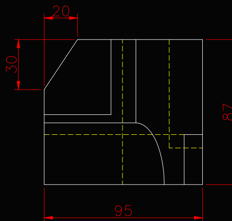
RIGHT SCALE 1/2
