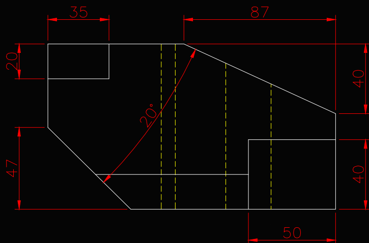
TOP SCALE 1/2
