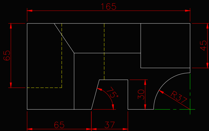
FRONT SCALE 1/2
