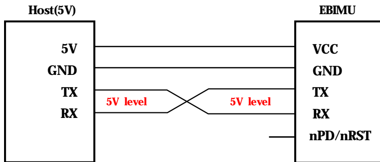
5V interface
