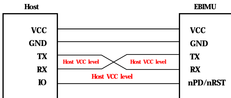
nPD/nRST connection
