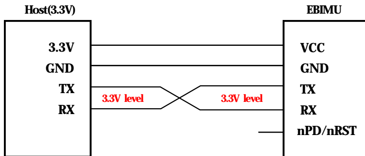
3.3V interface
