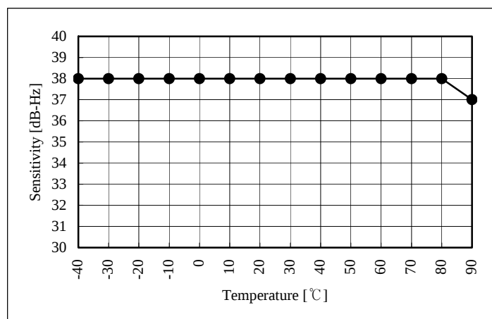
Temperature &amp; Sensitivity (Input : -130dBm)
