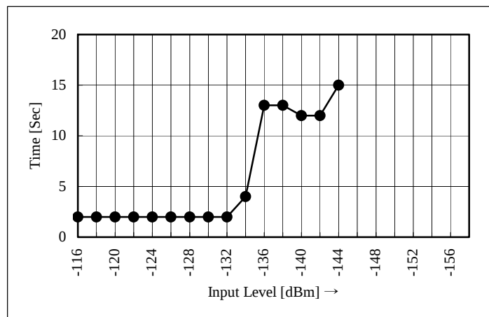
Re-Acquisition Time (After 5 Sec)
