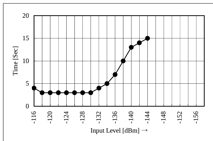
Re-Acquisition Time (After 60 Sec)
