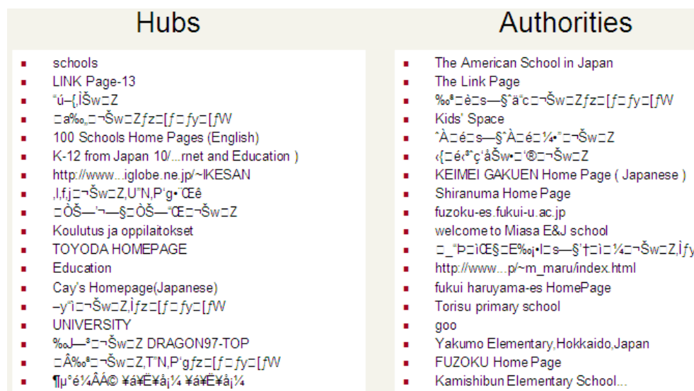
► Figure 21.6 A sample run of HITS on the query japan elementary schools.
