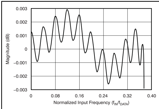
Figure 29. FIR Passband Amplitude Response ( f_{\text{DATA}} = 500\text{Hz} )
