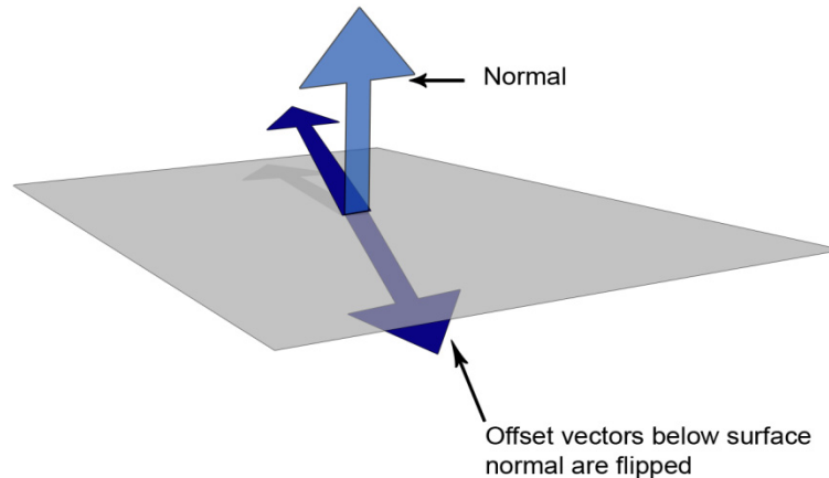
Figure 12. Handling self-occlusion.
