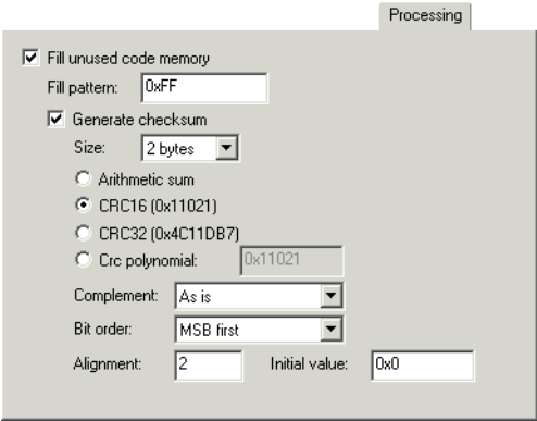
Figure 195: XLINK processing options
