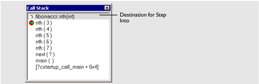
Figure 156: Call Stack window
