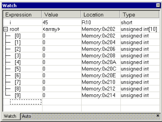
Figure 147: Watch window
