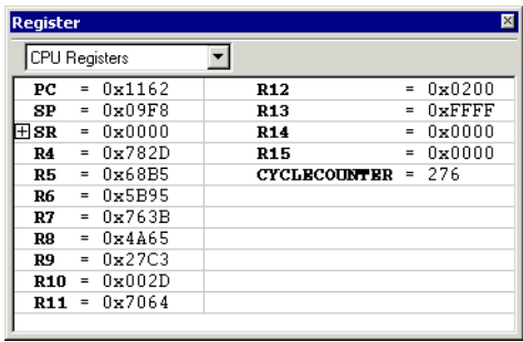
Figure 15: Register window
