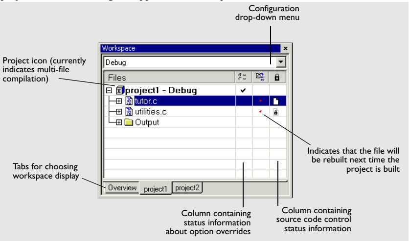
Figure 74: Workspace window
