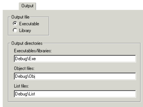
Figure 172: Output options
