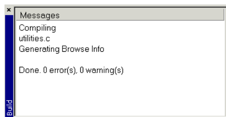
Figure 6: Compilation message
