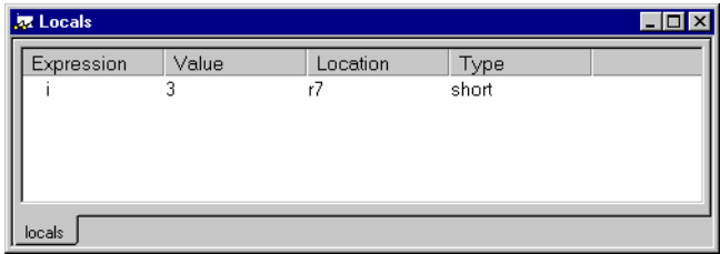
Figure 149: Locals window
