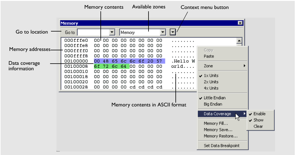
Figure 139: Memory window
