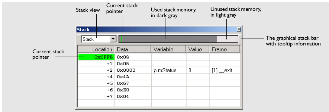
Figure 43: Stack window
