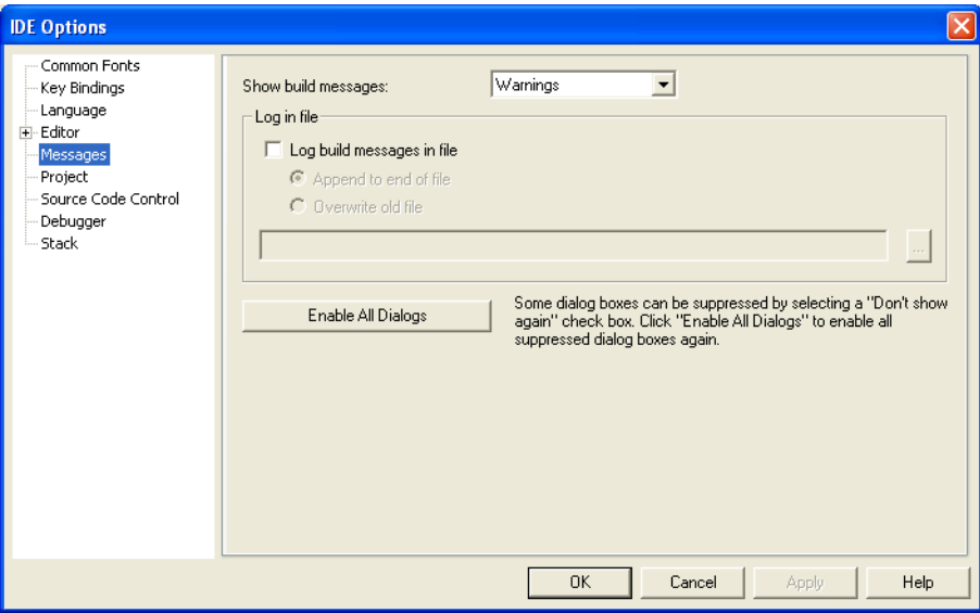
Figure 119: Messages option
