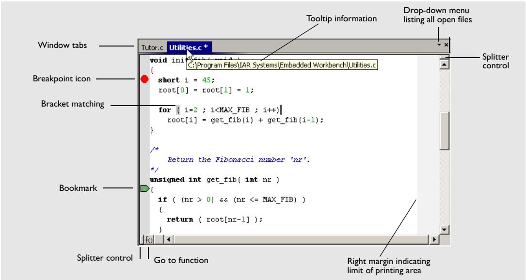
Figure 31: Editor window
