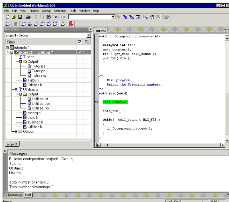
Figure 9: The C-SPY Debugger main window
