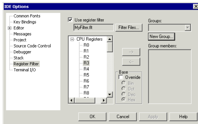
Figure 45: Register Filter page
