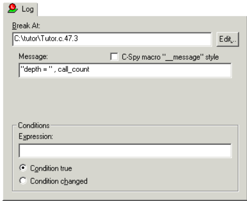
Figure 88: Log breakpoints page
