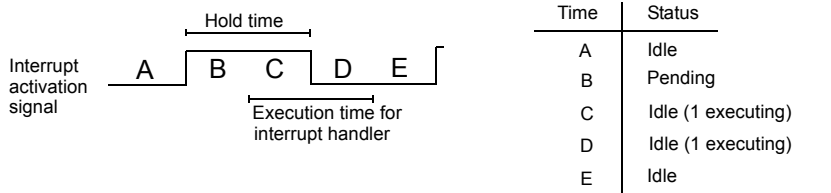
Figure 65: Simulation states - example 1
