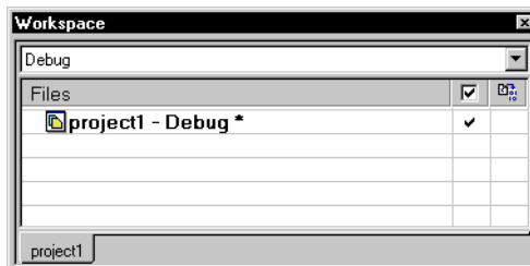
Figure 2: Workspace window
