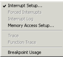
Figure 52: Simulator menu
