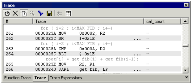
Figure 53: Trace window
