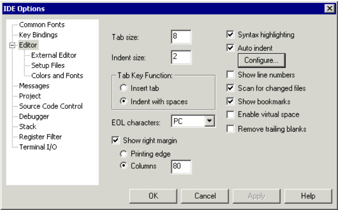
Figure 114: Editor options
