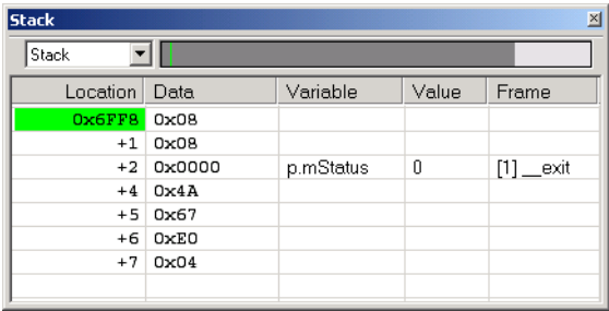
Figure 165: Stack window
