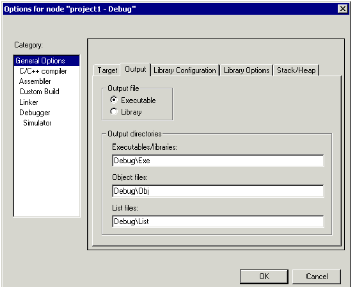
Figure 30: General options
