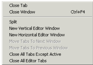
Figure 134: Window menu
