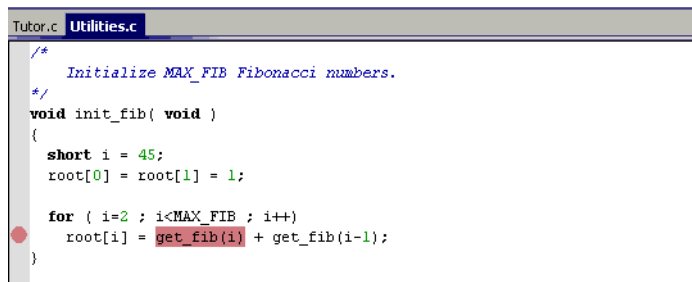
Figure 14: Setting breakpoints
