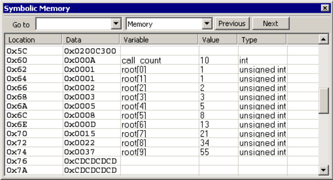
Figure 144: Symbolic Memory window
