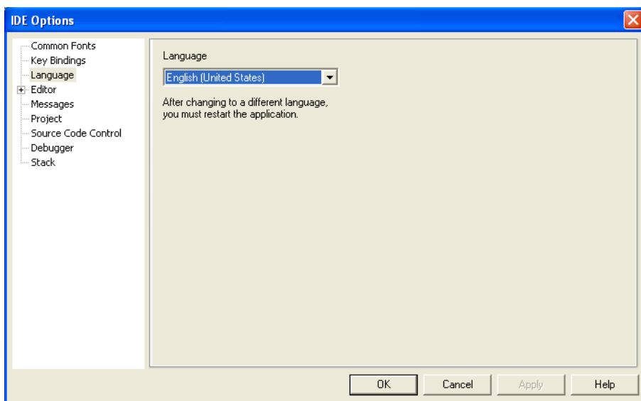
Figure 113: Language options
