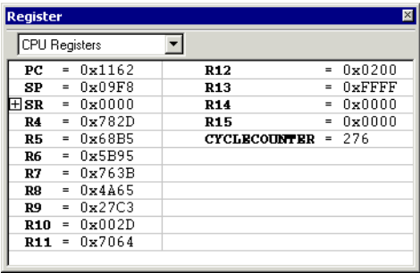
Figure 146: Register window
