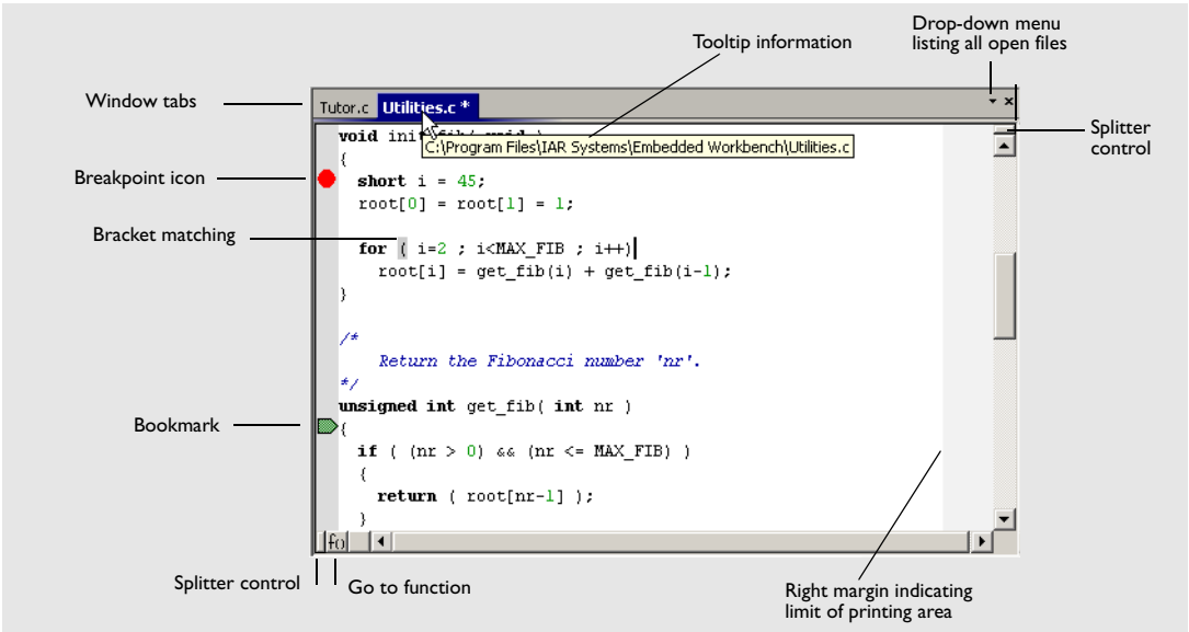
Figure 80: Editor window
