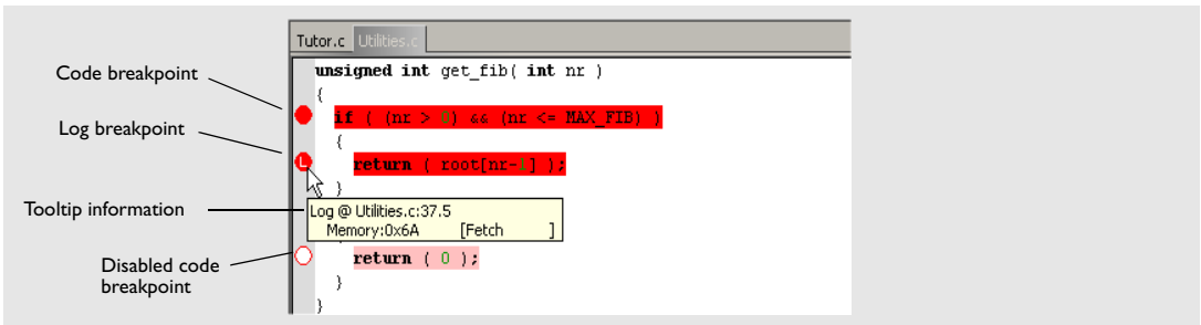
Figure 40: Breakpoint icons
