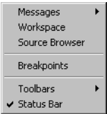
Figure 103: View menu
