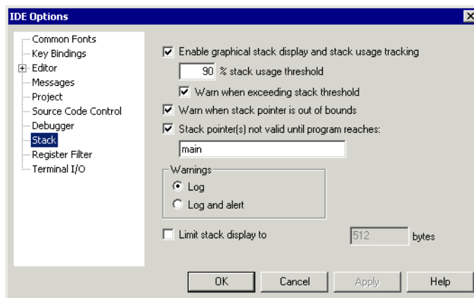
Figure 124: Stack options
