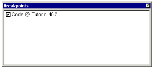
Figure 85: Breakpoints window
