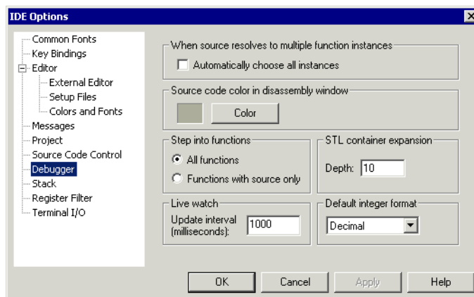
Figure 123: Debugger options
