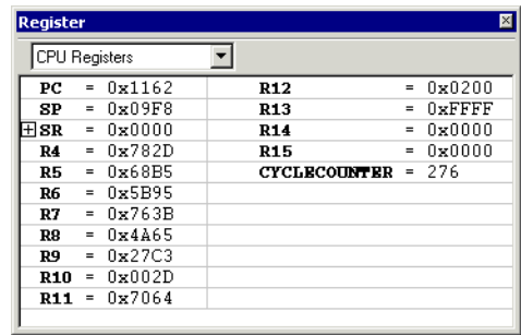
Figure 44: Register window
