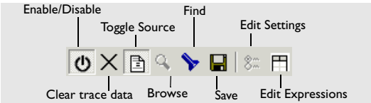
Figure 54: Trace toolbar
