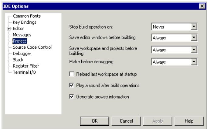
Figure 121: Projects options
