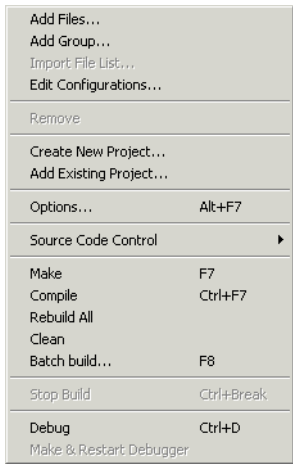
Figure 104: Project menu
